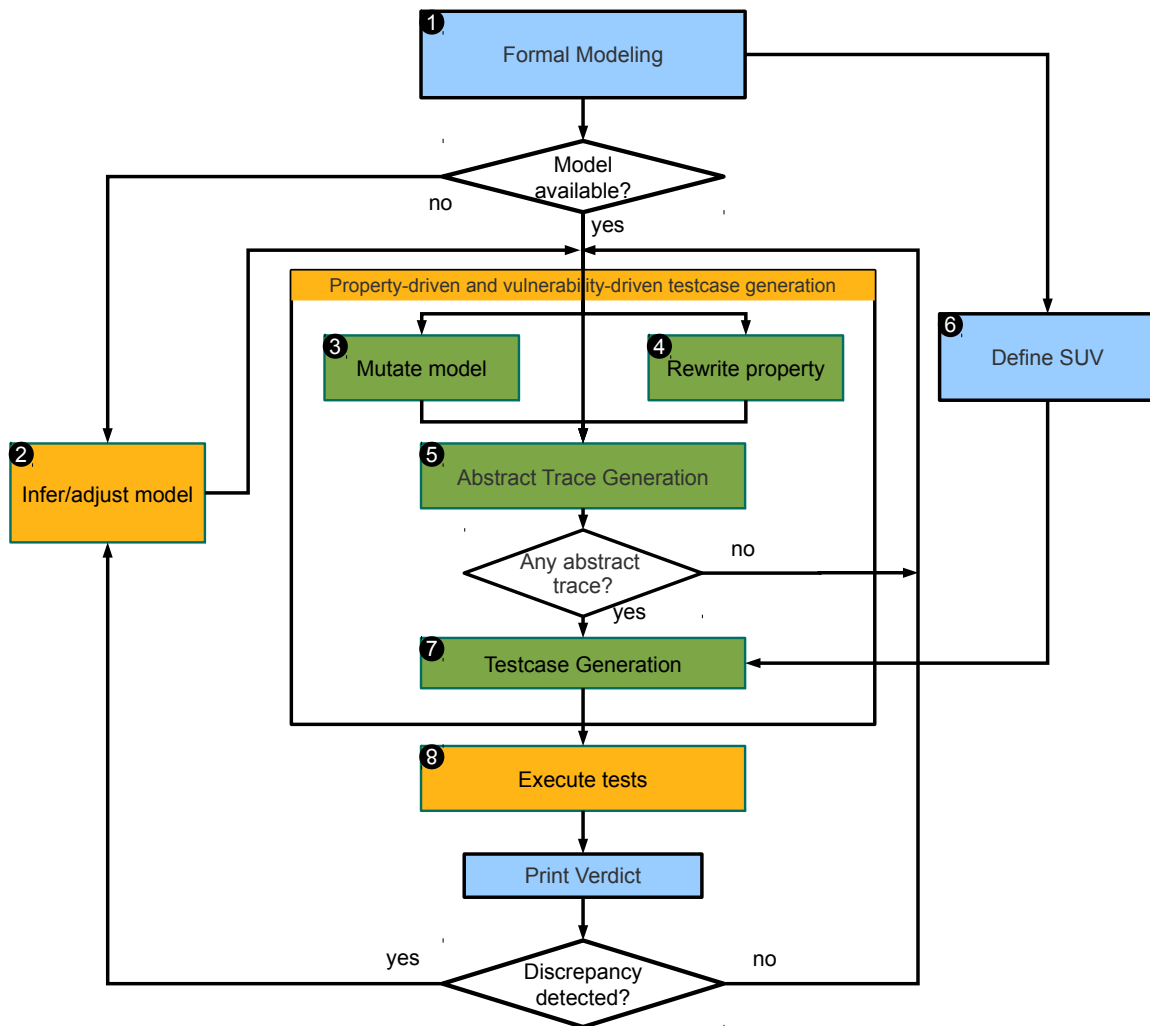
Figure 3: Interaction between the Security Analyst, the SPaCIoS Tool, and the SUV
